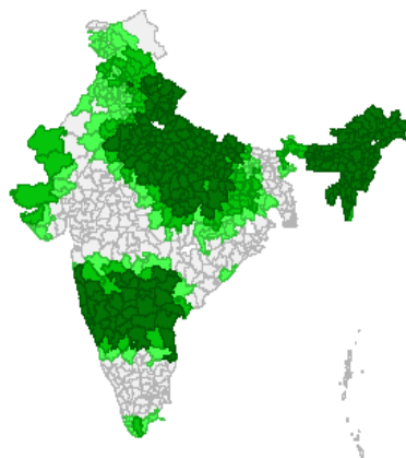
LISA Significant Map
