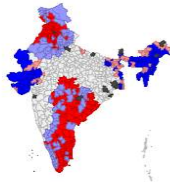
LISA Cluster Map
