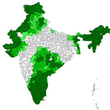
LISA Significant Map
