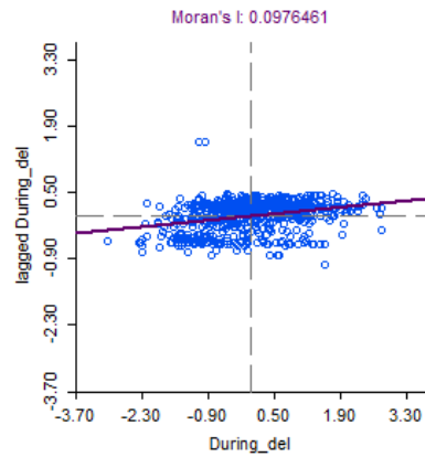
Moran Scatter Plot
