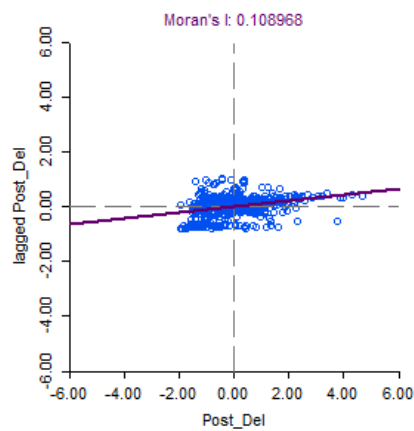
Moran Scatter Plot
