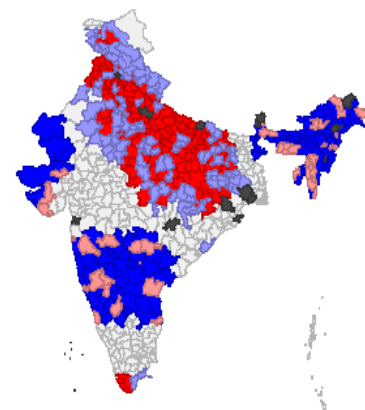
LISA Cluster Map
