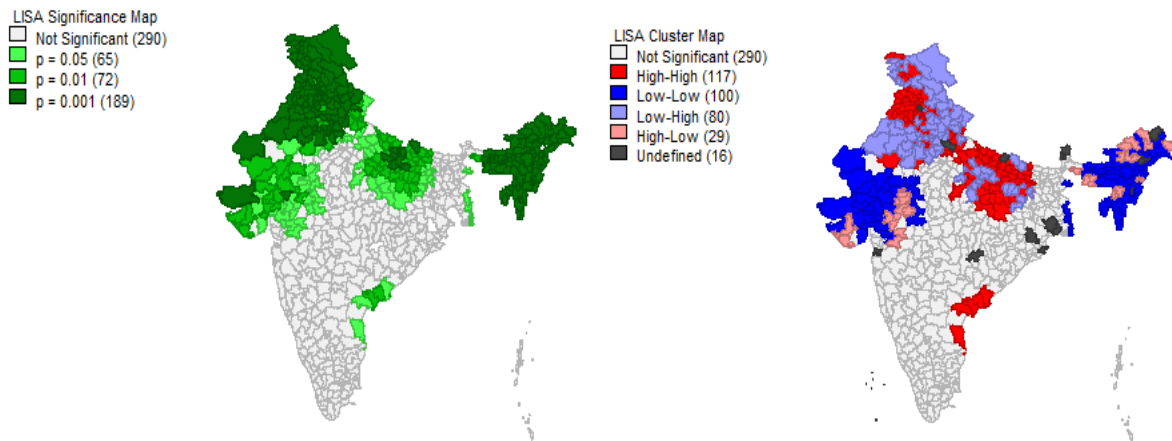
LISA Significant Map
